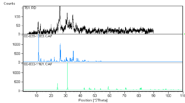
Fig. 3- XRD pattern of the ammonium-sulfate-modified clinoptilolite compared to the CAF.1383-039-00 card for Raw clinoptilolite and the CAF.1161-033-00 card for Quartz
