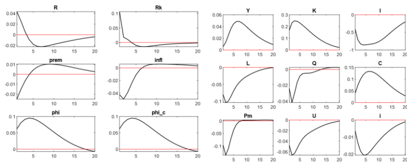
Figure 5. Response of selected variables to a capital quality shock
