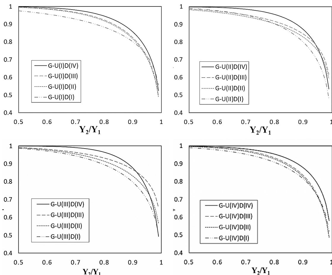
Fig. 6-Relation of ( \psi ) with ( Y_2/Y_1 ) for different up and downstream slopes
