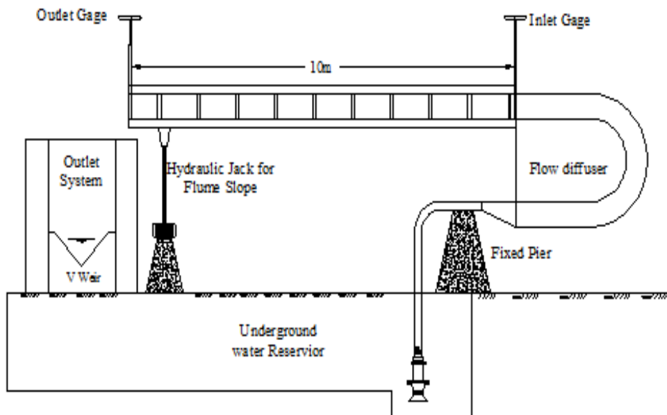
Fig. 1- Plan view of the experimental flume
